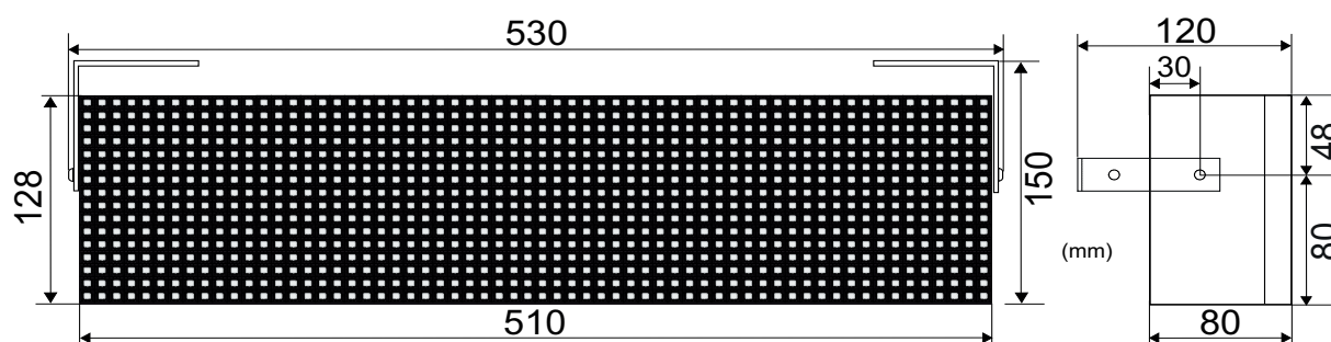
Fig. 2 Dimensions DISBRSE
