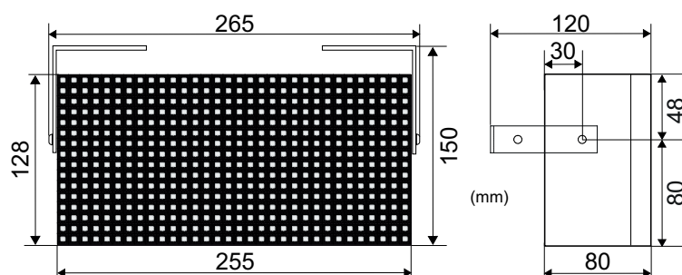
Fig. 1 Dimensions DISARSE
